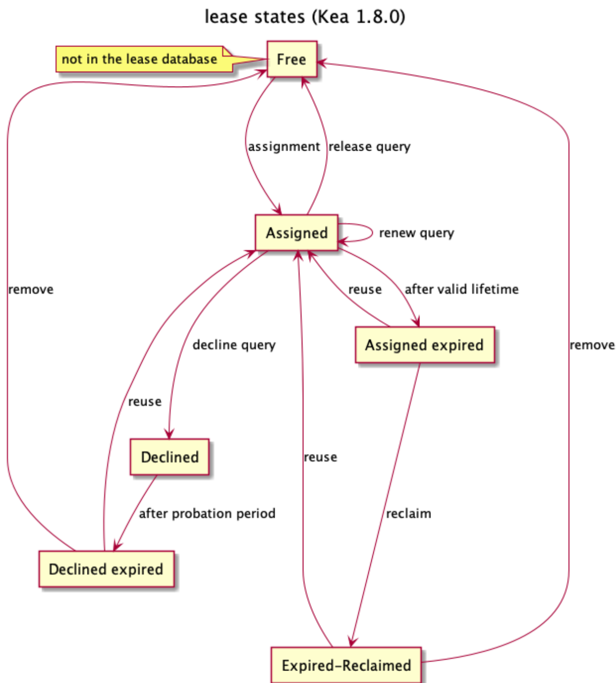
Fig. 8: Lease states
