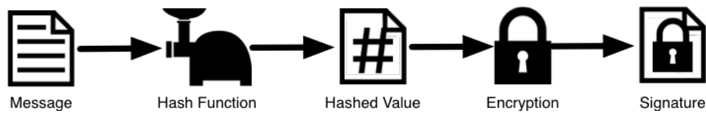
Fig. 1: Signature Generation
